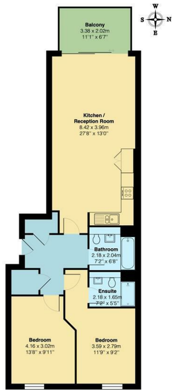
Second Floor Total Area: 75.2 m 2 ... 809 ft 2 (excluding balcony) All measurements are approximate and for display purposes only
